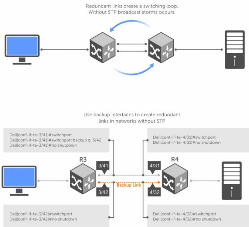
Figure 64. Configuring Redundant Layer 2 Pairs without Spanning Tree
